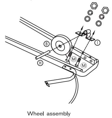
Wheel assembly
